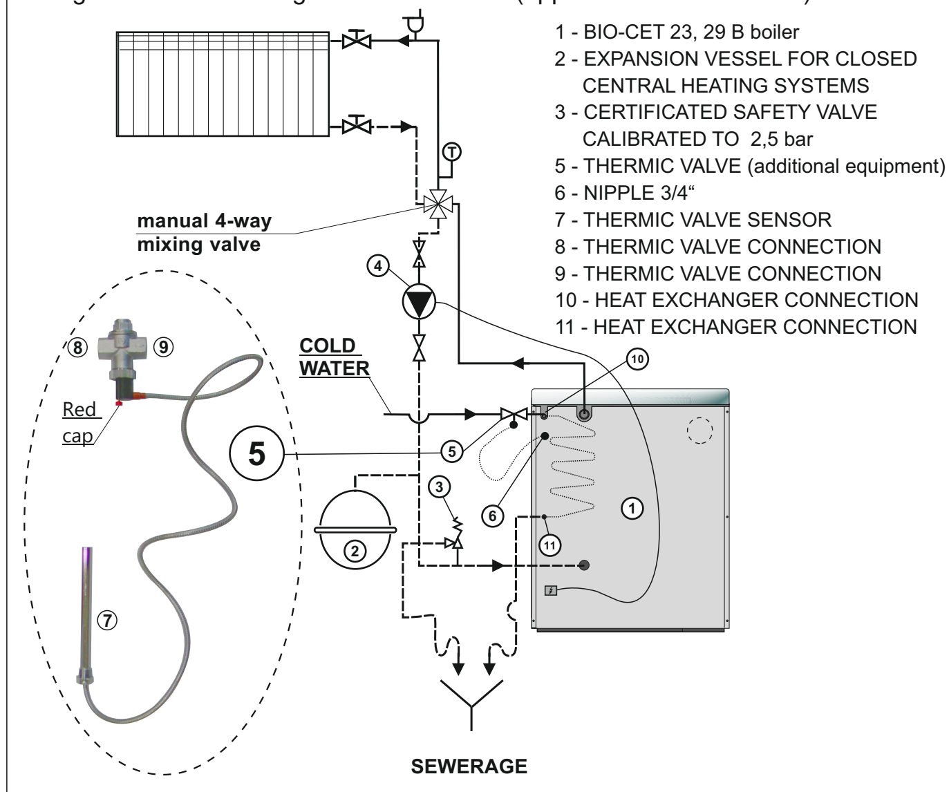
Diagram 2. - Connecting an BIO-CET B - L (applies to BIO-CET B - D)
